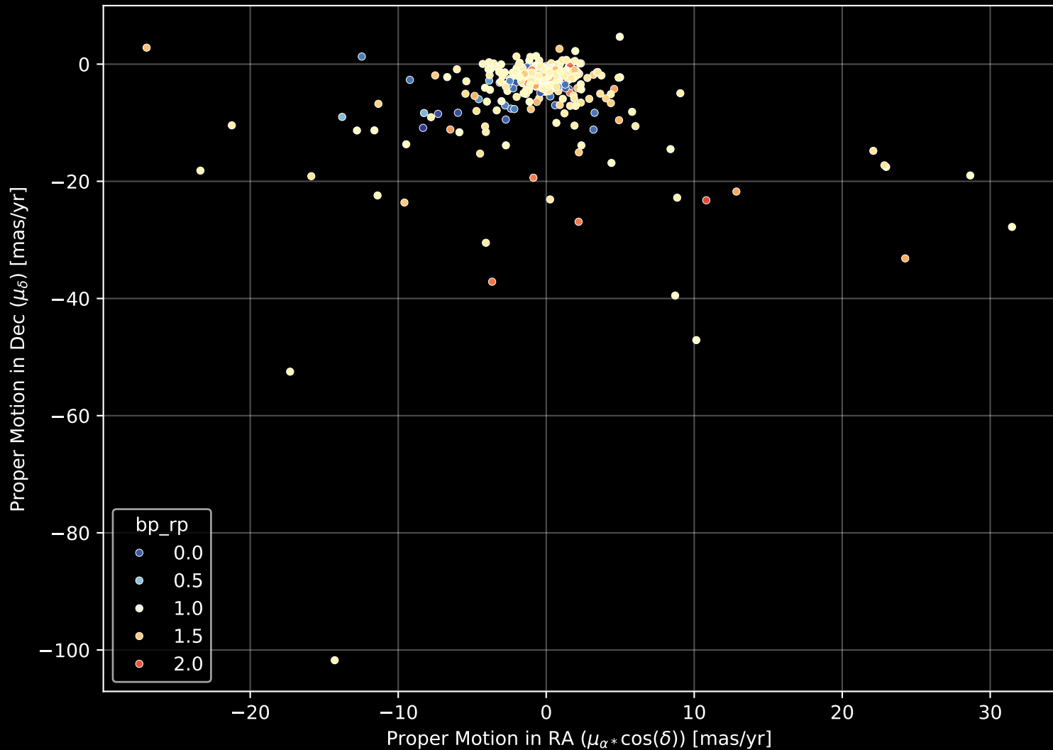
APOGEE DR17 Field: [191+12] Proper Motion Diagram (n= 331)
