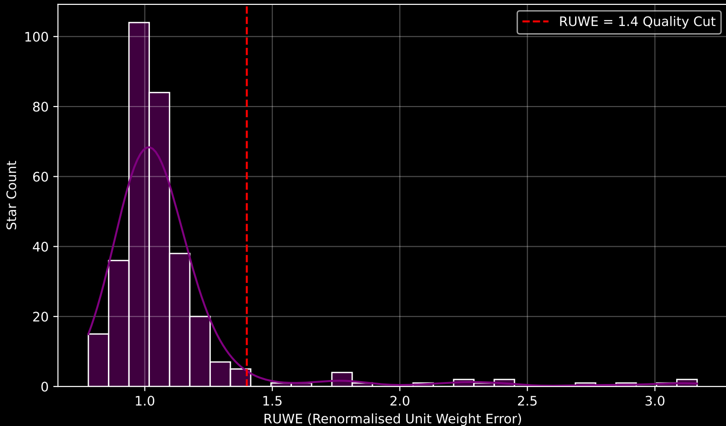
GAPOGEE DR17 Field [191+12] RUWE Distribution (n= 327)
