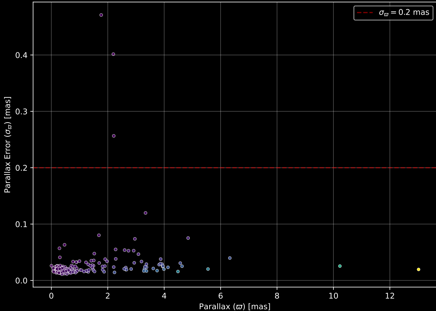
APOGEE DR17 Field: [191+12] Parallax Quality (n= 331)
