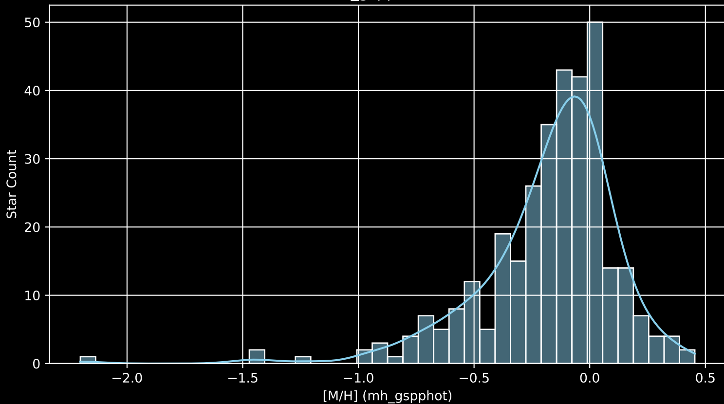
APOGEE DR17 Field: [191+12 [M/H] (mh_gspphot) (n= 326)
