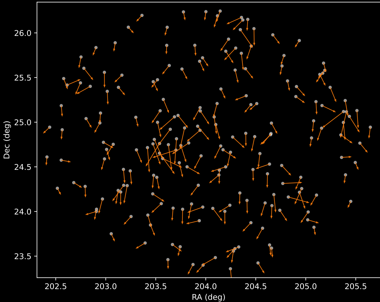
APOGEE DR17 Cluster 2 Proper Motion Vectors (n=192)
