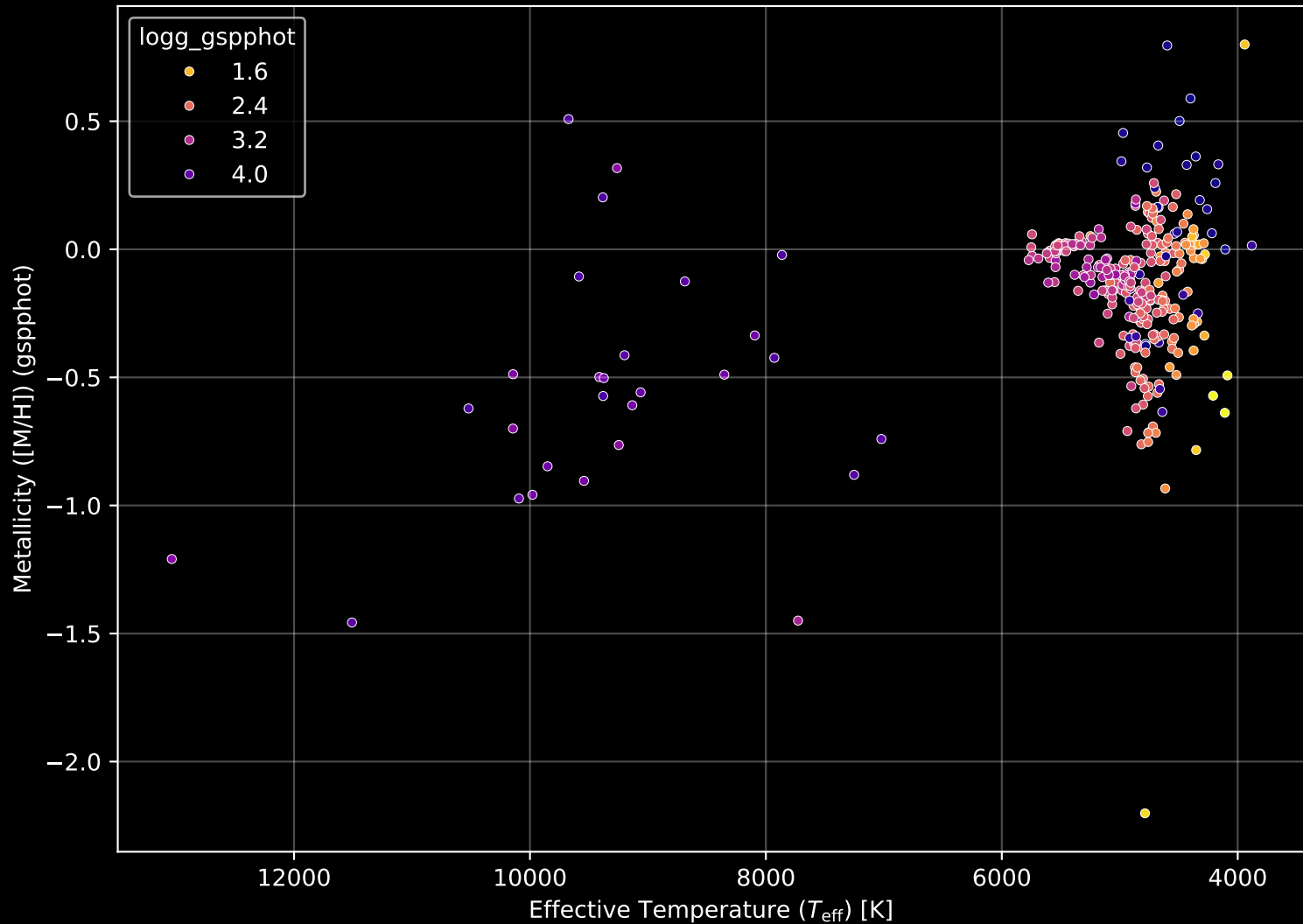
APOGEE DR17 Field: [191+12] Stellar Population Parameters (n= 331)
