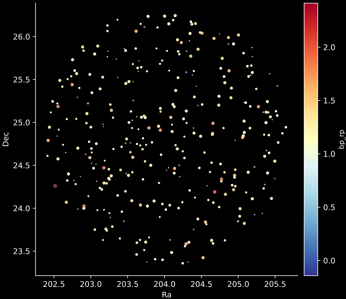
APOGEE DR17 Field: [191+12] Stars: 331
